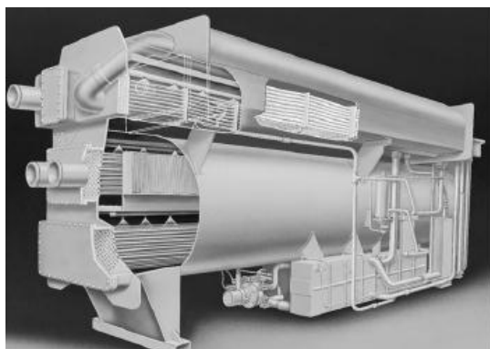
Figure 6.2 Machine à Absorption LiBr (Trane)
