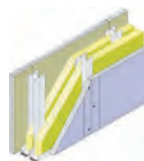
Cloison séparative SAD 160 Placo® DuoTech® 25 R_w (C; C_{tr}) = 69 (-3; -10) \text{ dB}
